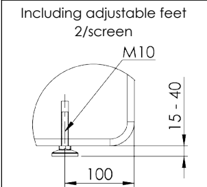
Section view of ScreenIT A30 straight corners
