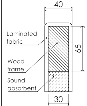
Section view of ScreenIT A30 straight corners
