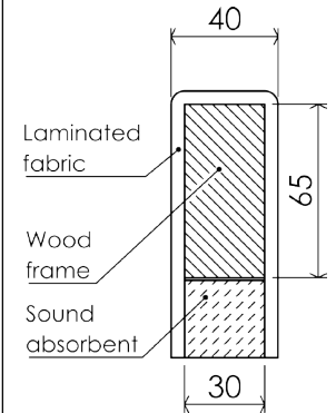
Section view of ScreenIT A30 straight corners
