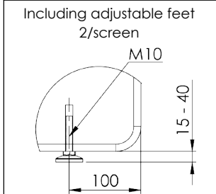
Section view of ScreenIT A30 straight corners
