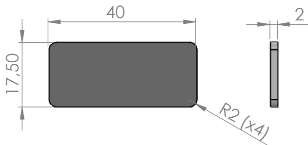
Support plate 1:1
