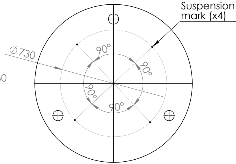
Suspension mark
