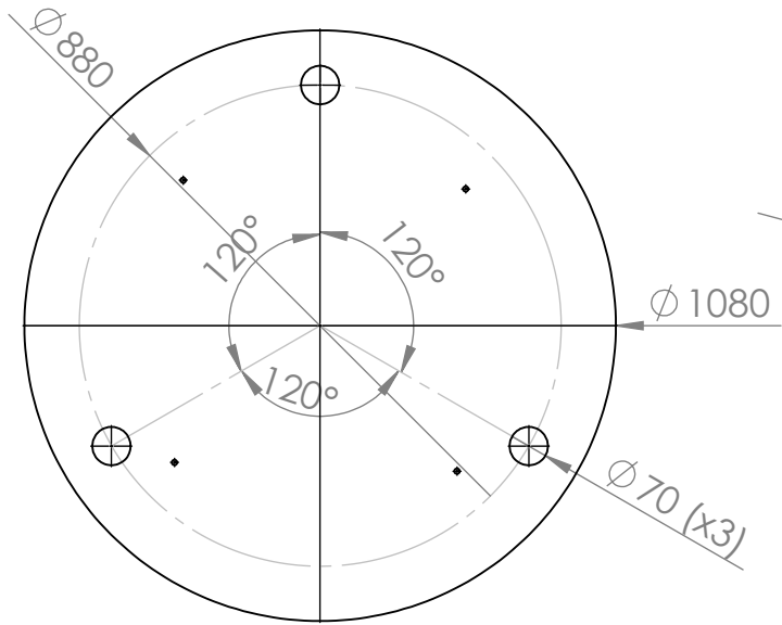
Lamp holes
