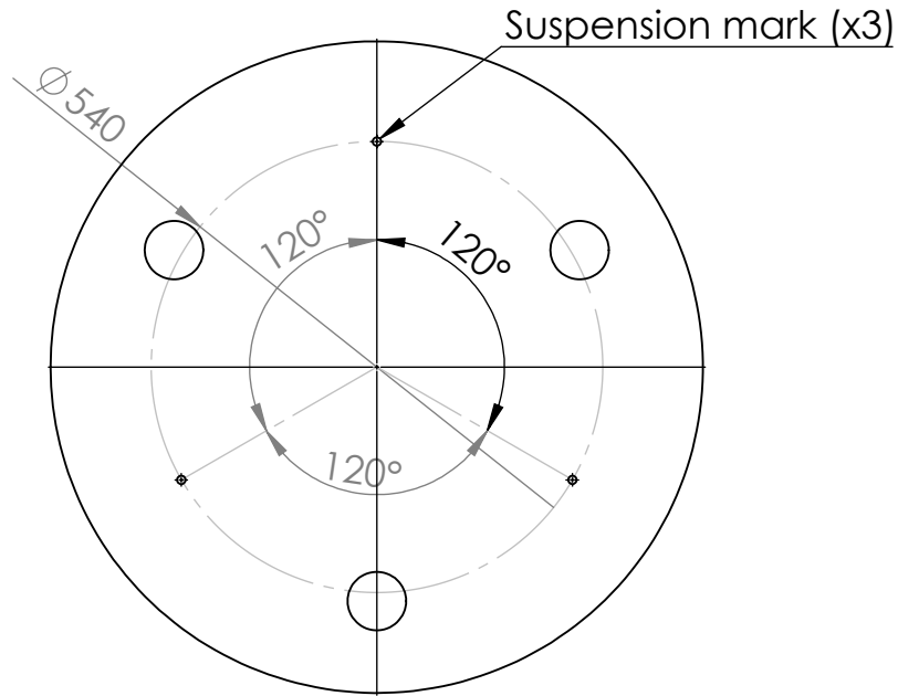
Suspension mark
