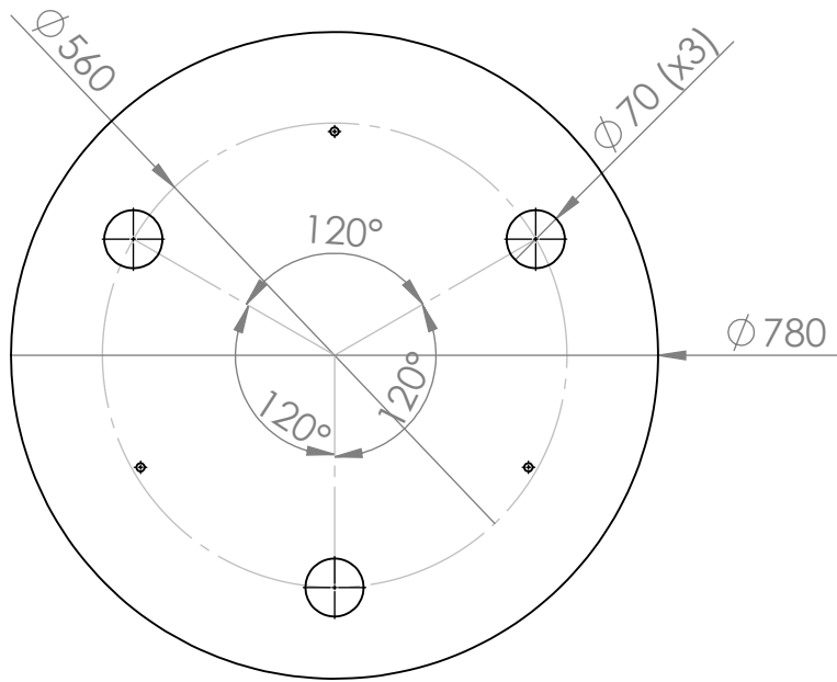
Lamp holes
