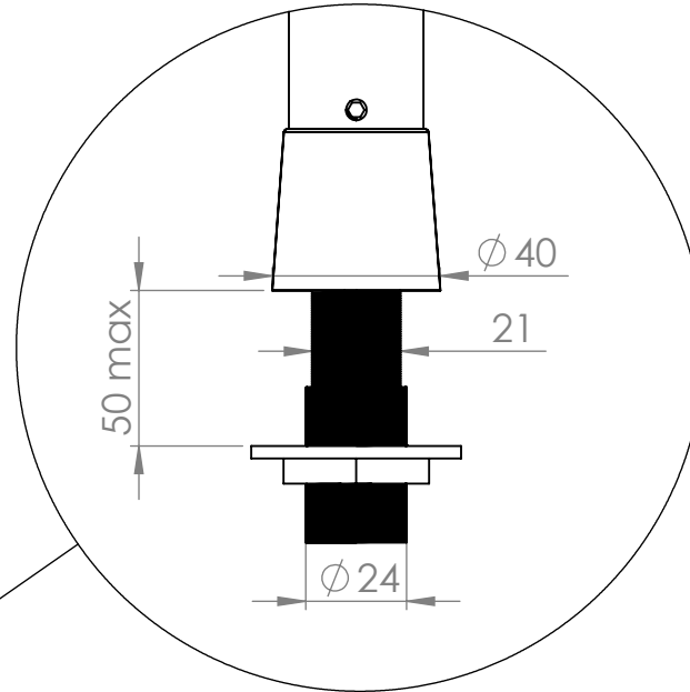
DETAIL D SCALE 1 : 2
